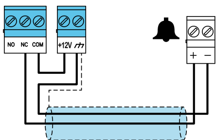
2 wire connection
