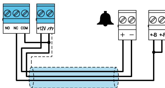
3 wire connection
